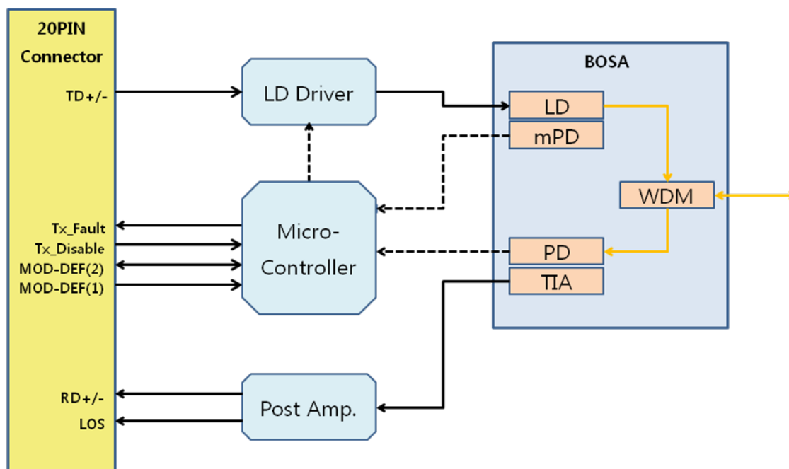
Fig. 1 Block Diagram
