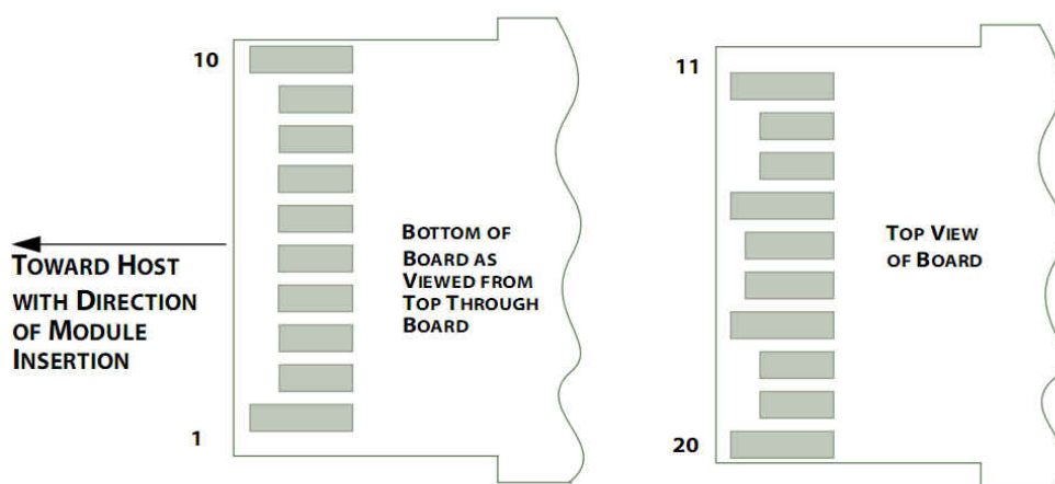
Fig. 2 SFP+ Transceiver Electrical Pad Layout
