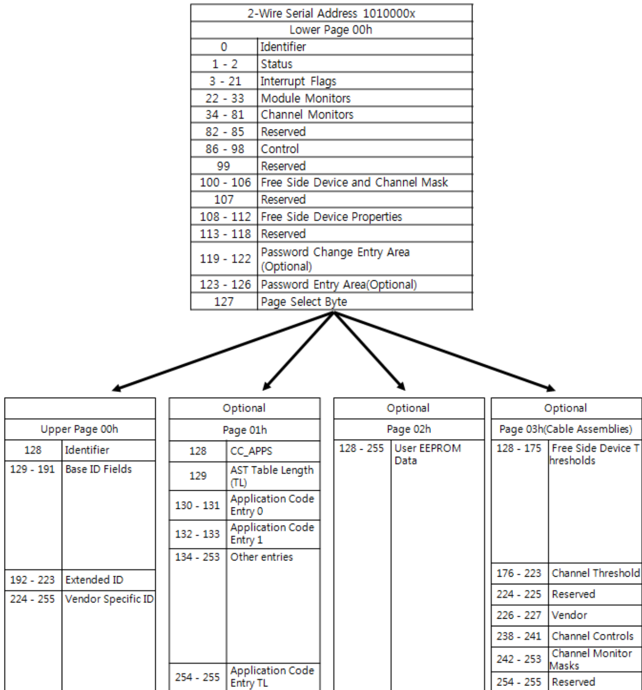
Fig 7. Memory map
